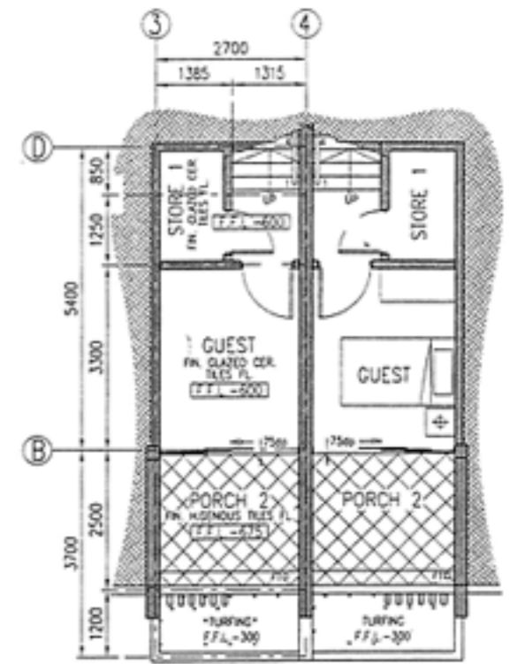
Type A Lower Ground Floor Plan
