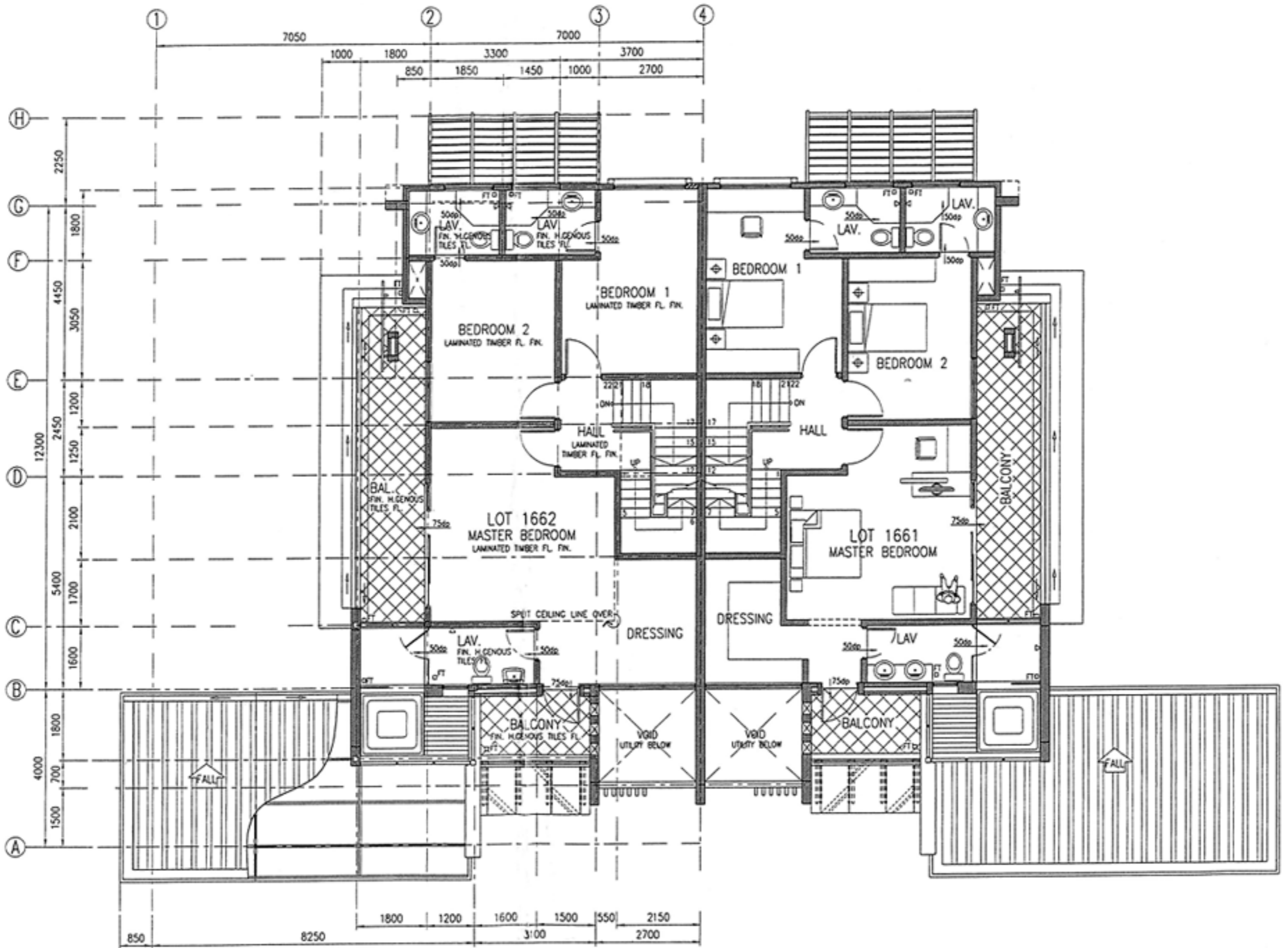
Type A First Floor Plan
