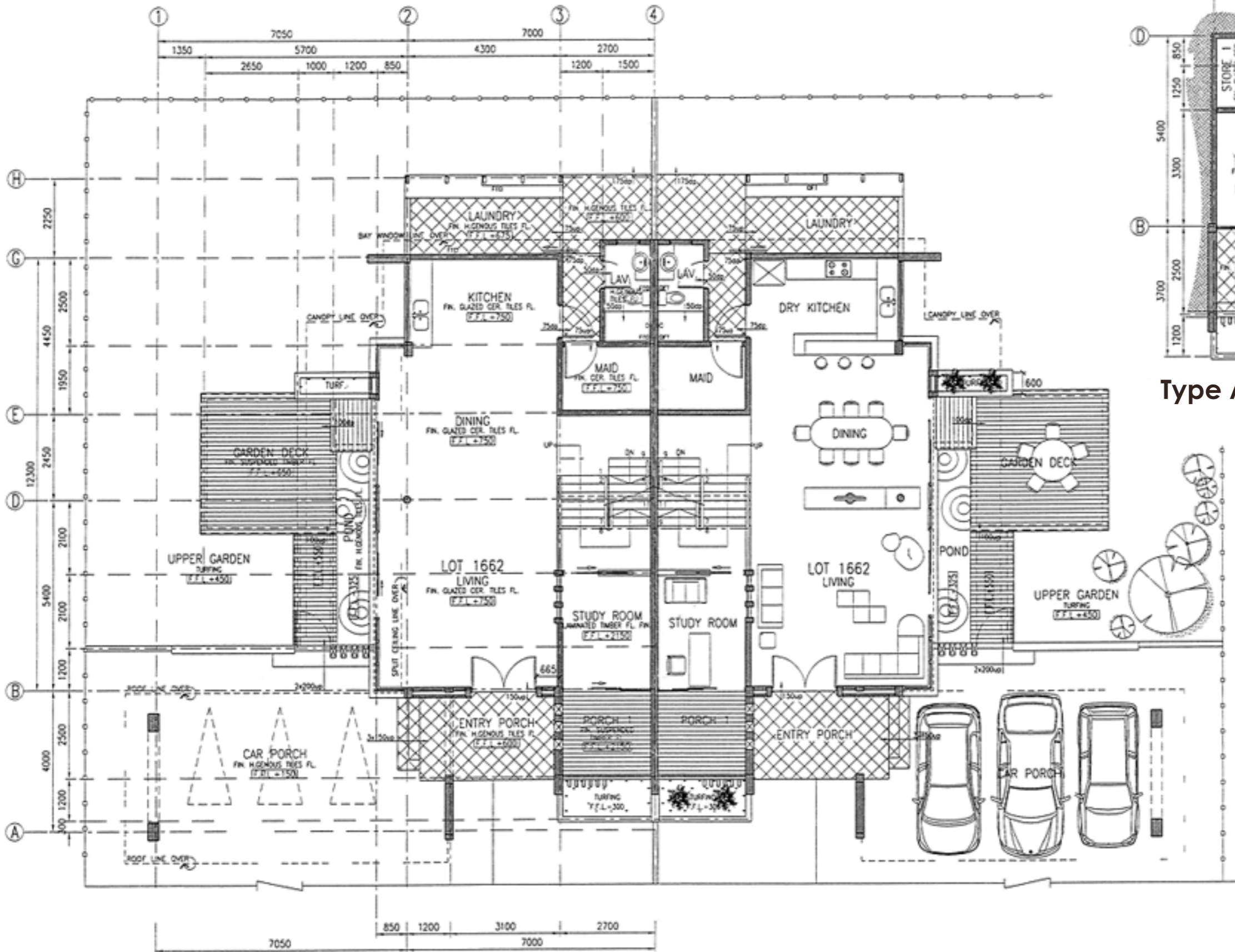
Type A Ground Floor Plan
