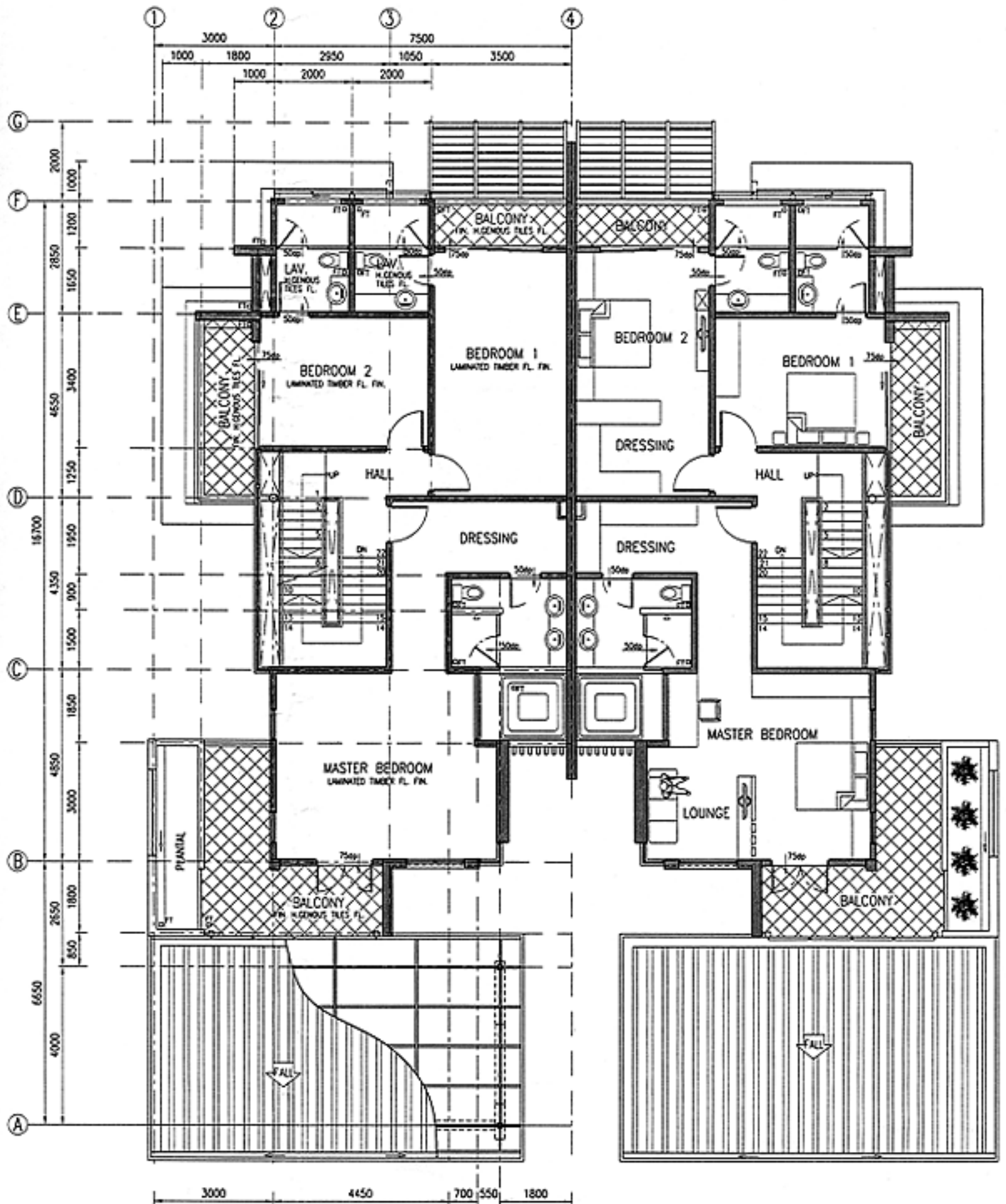
Type B First Floor Plan
