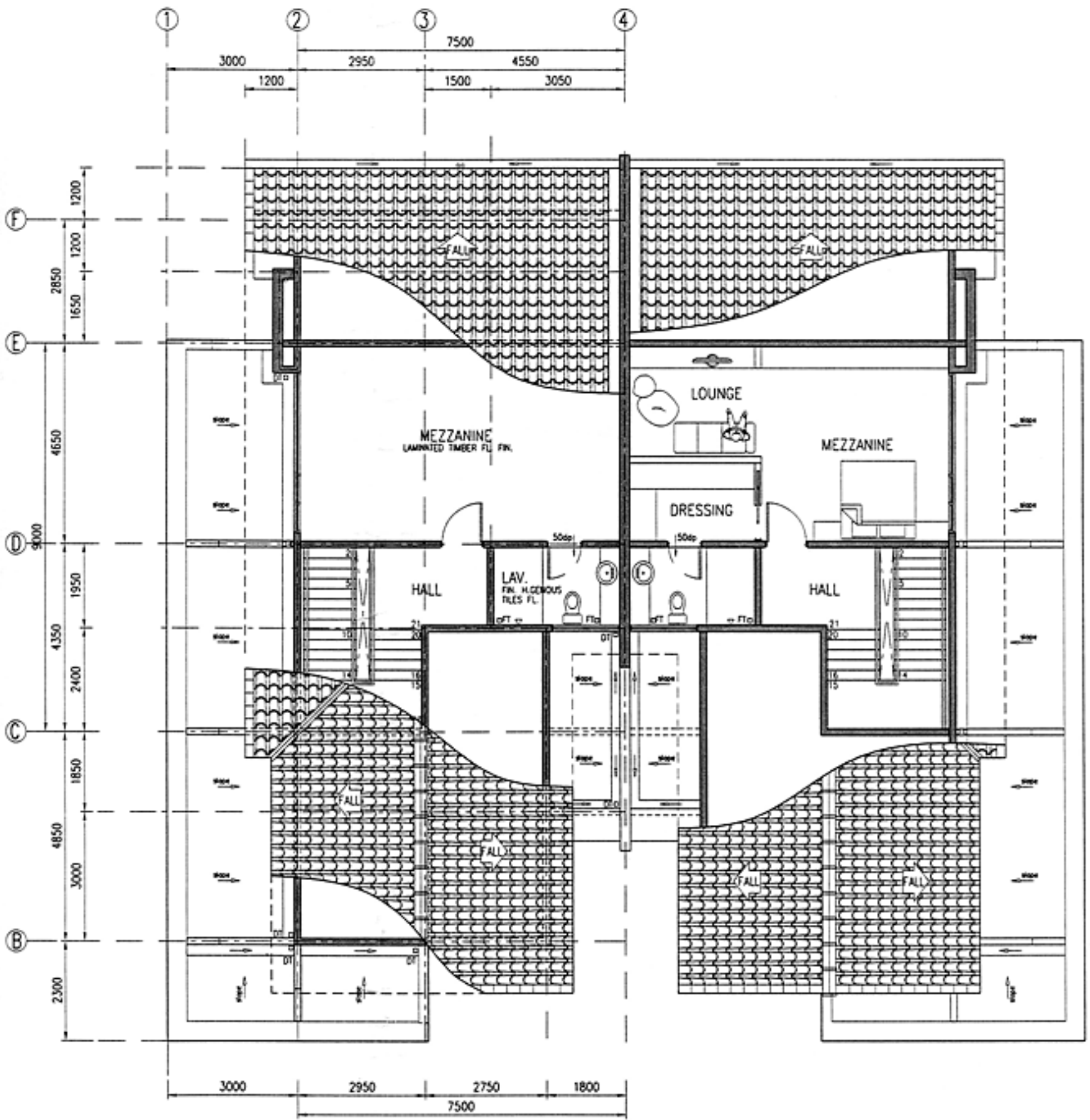
Type B Mezzanine Floor Plan
